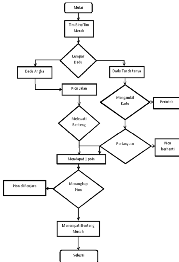
Gambar 5. Flowchart "RATON"
